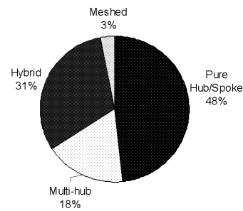
Fig. 18. Structural classification of all VPNs
